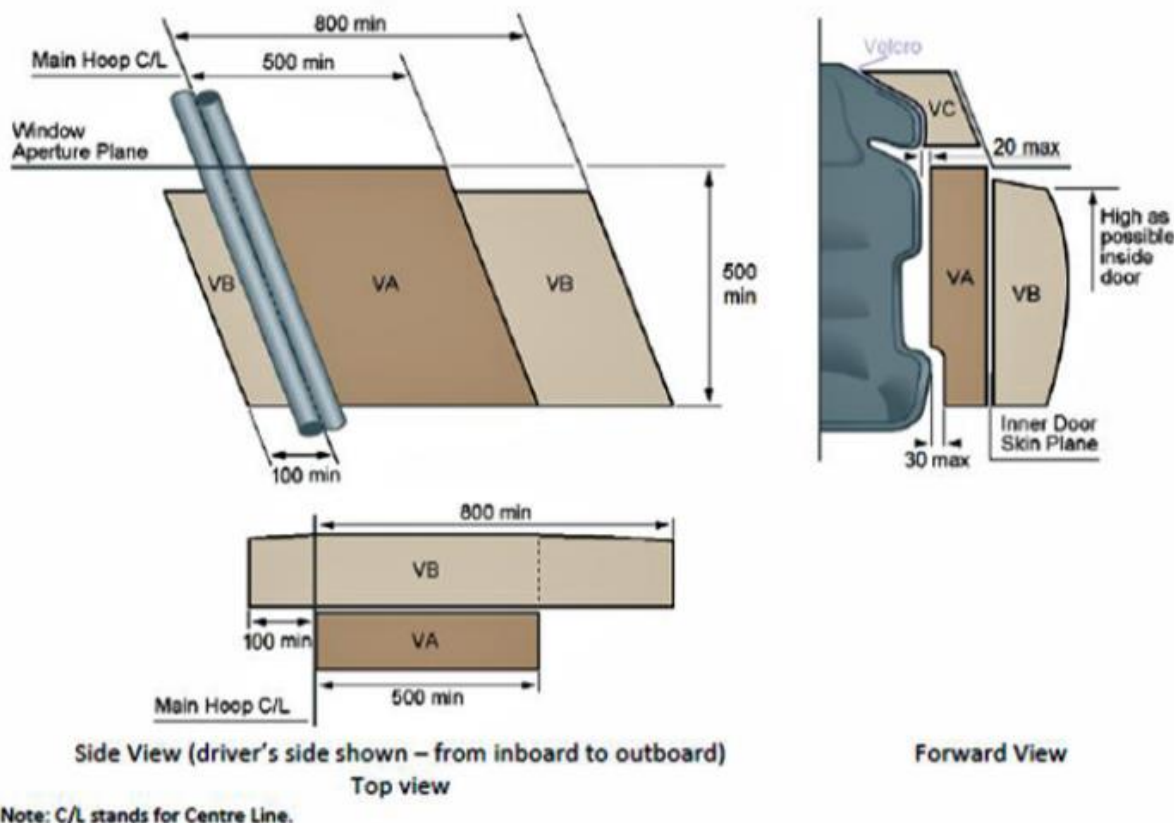
Figure 1. Minimum geometry for door foam and head foam volumes
